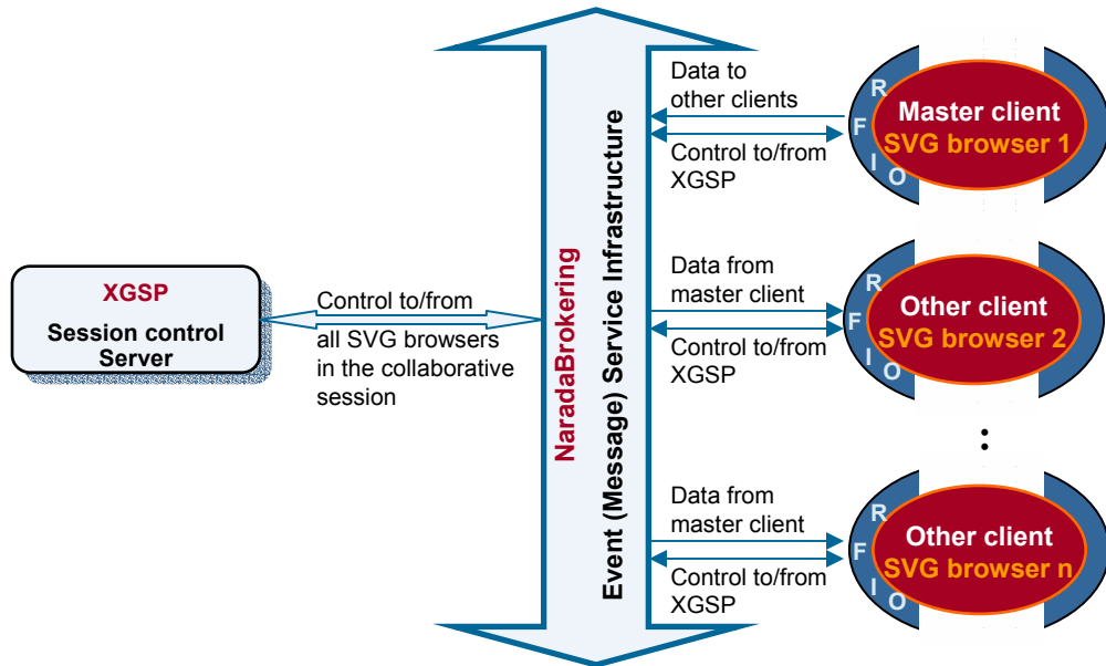
Figure 3 Architecture of collaborative SVG browser on PC
